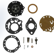
5075 | Tillotson Stihl 08/ P840/P835 Cod Fab: -
