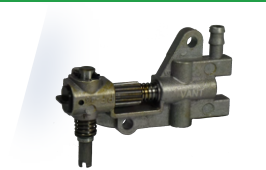
4| MS 45/52 CPL Cod Fab: KWS-455200-182
