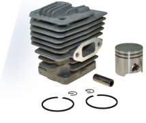
6300| Stihl FS220 CPL 38mm
